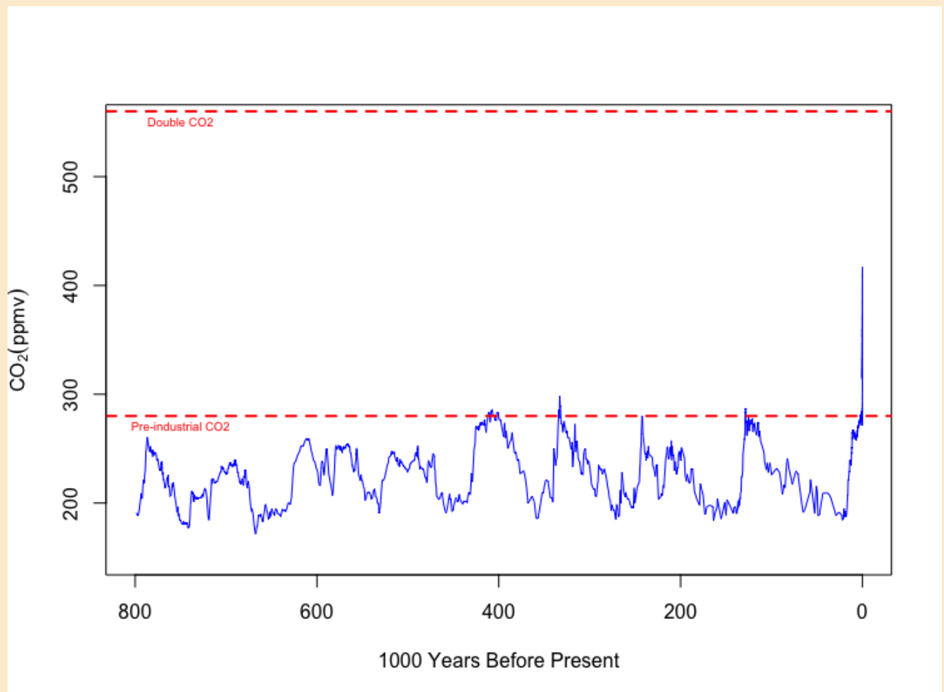
Figure 2b. A graph showing the past 800,000 years of atmospheric carbon dioxide concentration. CO 2 data after 1958 are from the Scripps CO 2 program (Keeling et al. 2001), CO 2 data from 1958 to 2000 years before present are from MacFarling Meure et al. (2006) and older CO 2 data back 800,000 years are from Lüthi et al. (2008).
