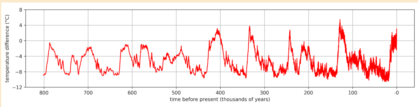
Figure 2a. Temperature reconstruction for Antarctica for the past 800,000 years. Data source: Jouzel et al. (2007).
