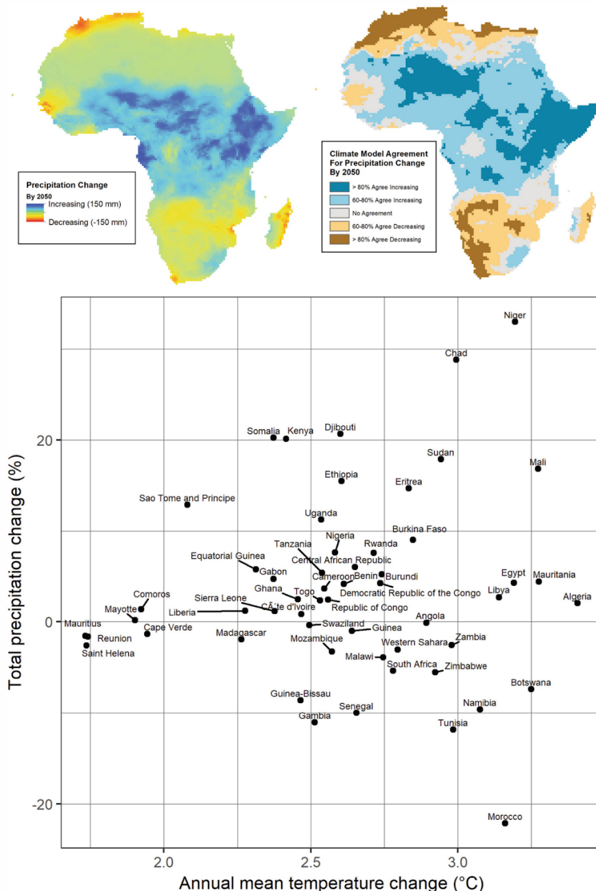
Figure 3. Climate model projections for Africa by 2050. Top left: Projected total annual precipitation changes, using data from the median Coupled Model Intercomparison Project Phase 5 (CMIP5) under RCP8.5. Top right: CMIP5 model projections for future precipitation changes do not always agree; the regions for which model projections are in greatest agreement are shaded dark brown (decreased rainfall in Northern and Southern Africa) and dark blue (increased rainfall across Central and East Africa). There is no overall consensus between the models of the magnitude of precipitation change. Bottom: The average change in precipitation and temperature, by country, in 2050, based on projections by multiple CMIP5 models. Source: Girvetz et al., 2018. (This image is reproduced under the terms of the Creative Commons Attribution 4.0 International License, http://creativecommons.org/licenses/by/4.0/ ).
